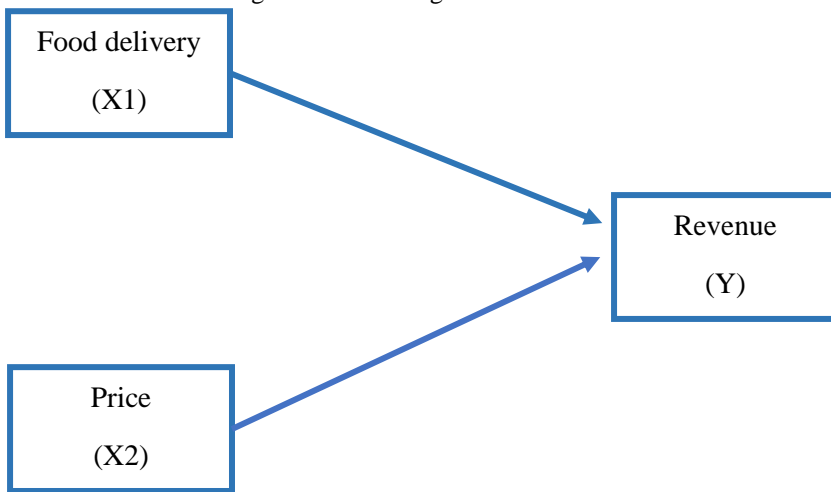
Figure 2. 4Thinking Framework
