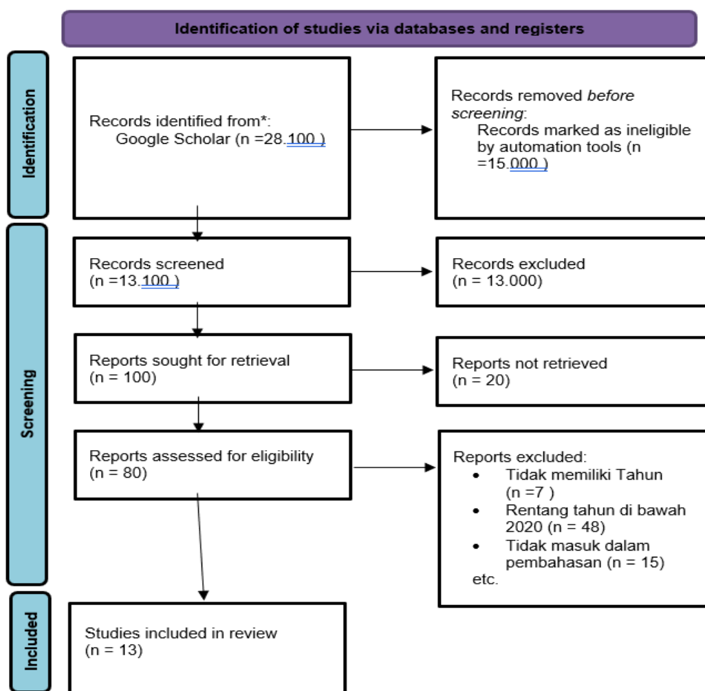
Gambar 1 : Diagram PRISMA
